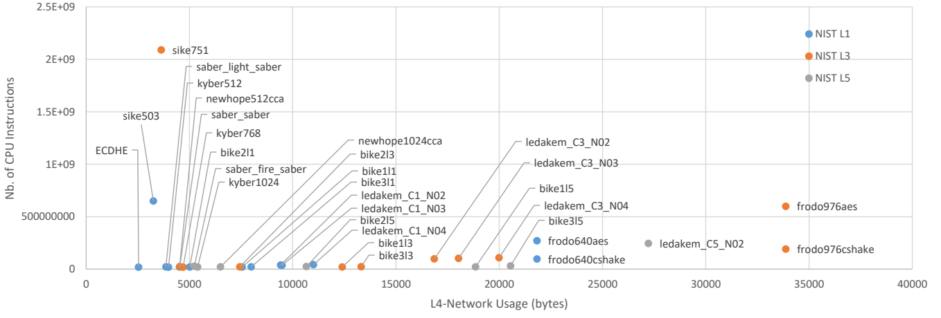
Fig. 3. Performance evaluation of native and hybrid PQ-KEX using TLS 1.3
