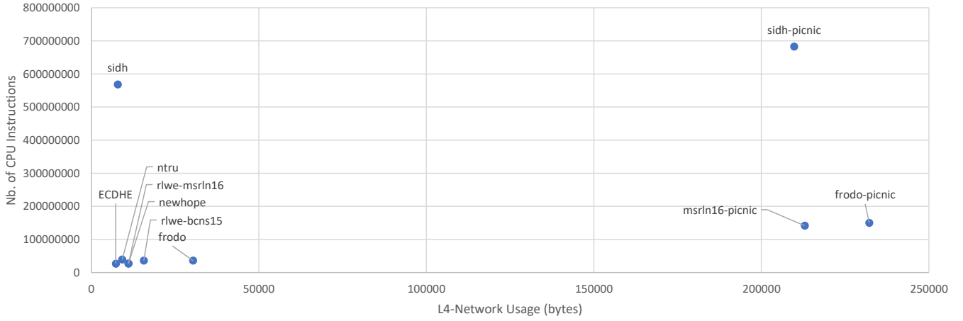
Fig. 2. Performance evaluation of PQ-KEX and PQ-SIGN using TLS 1.2 with default parameters of OQS-OpenSSL branch OpenSSL_1_0_2-stable.
