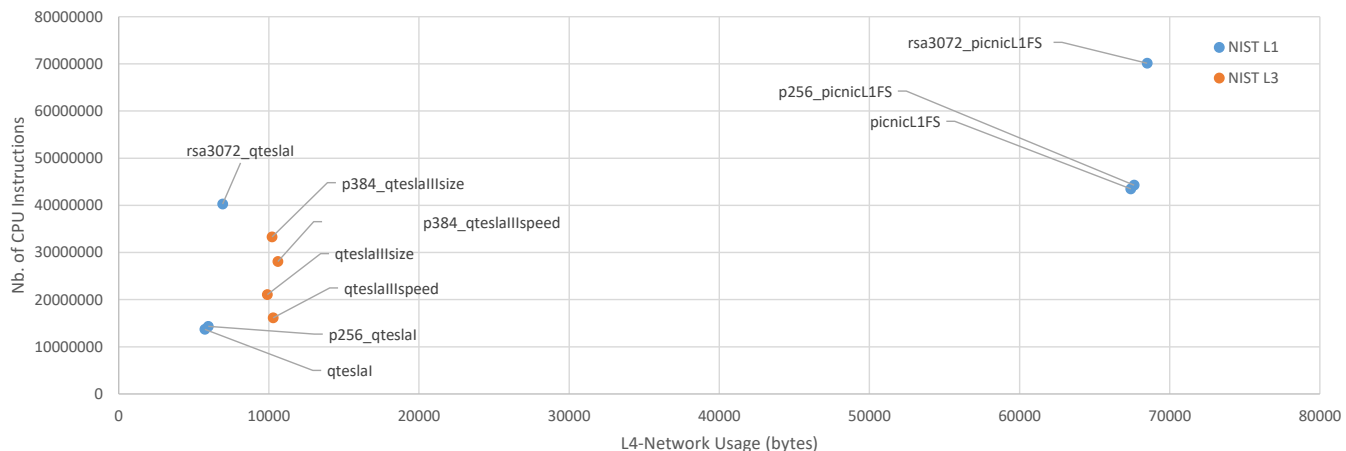
Fig. 4. Performance evaluation of native and hybrid PQ-SIGN using TLS 1.3
