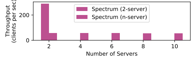
Figure 5: Spectrum can generalize to n > 2 servers (shown for 10 kB messages). This uses an expensive PRG and is therefore slower, but adding more servers causes no additional slowdown.
