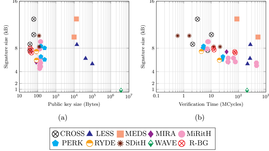
Fig. 8: Comparison between R-BG and code-based signature schemes from the NIST competition.
